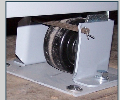
Caster Brackets
