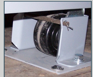
Caster Brackets
